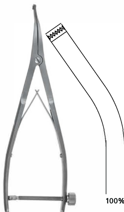
Inge lamina spreader curved with speedlock, short jaws RS 7545 - 8 / 280mm, spread 30mm
