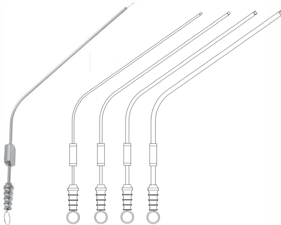
McCulloch suction tubes, working length 125mm, 55° RL 2045 - 1,7mm = 5 FR RL 2046 - 2,3mm = 7 FR RL 2047 - 3,0mm = 9 FR RL 2048 - 4,0mm = 12 FR
