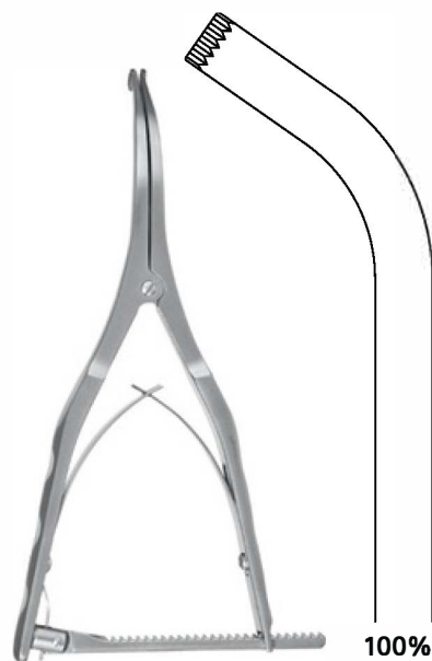
Inge lamina spreader curved jaw, with rack RS 7535 - 7 / 180mm, spread 34mm
